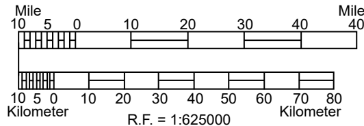
Figure 1.16: Comparative Scale
