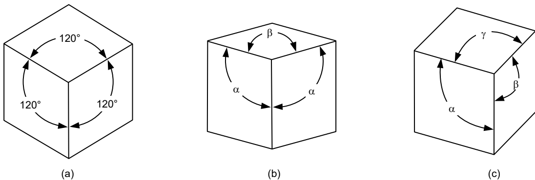
Figure 2.3: Isometric, Dimetric and Trimetric Projections
