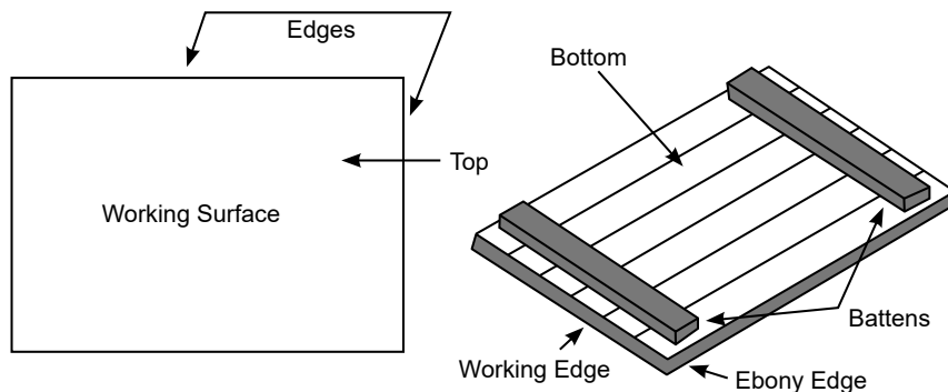
Figure 1.4: Drawing Board
