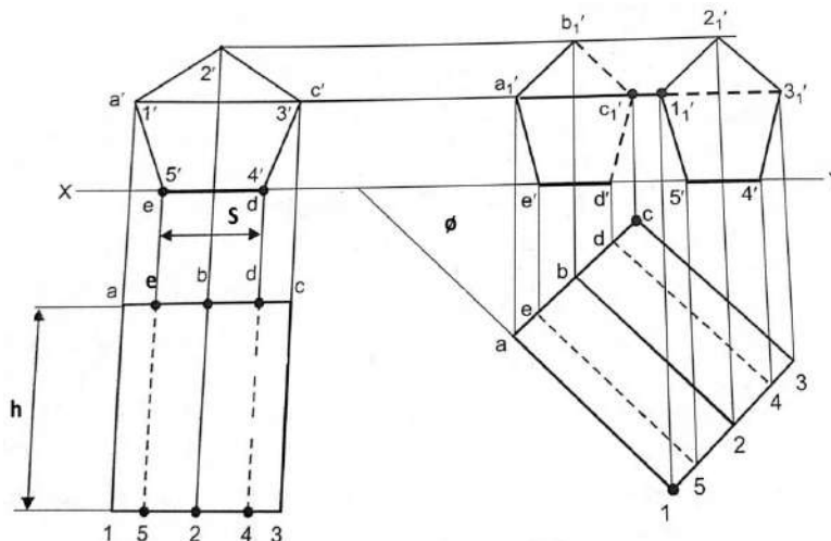
Figure 3.16: Projection of a Pentagonal Prism Axis parallel to HP and Inclined to VP
