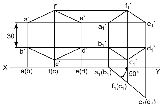
Figure 2.36: Projection of Hexagonal Plate
