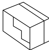
Figure 5.16 (c): Drawing Line Parallel to Isometric Axes
