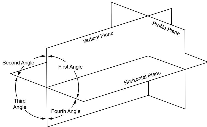
Figure 2.7: Principal Planes
