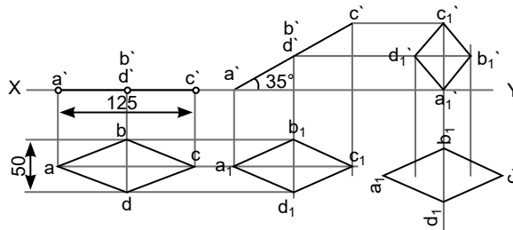
Figure 2.38: Projection of a Rhombus
