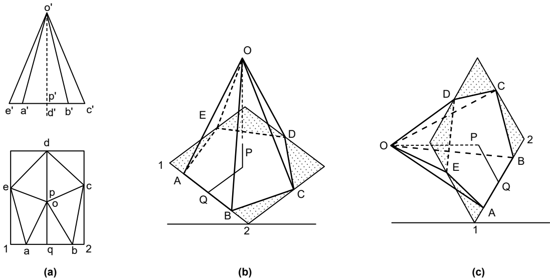
Figure 5.14: Isometric View of a Pentagonal Pyramid
