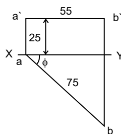
Figure 2.27: Projection of Line AB
