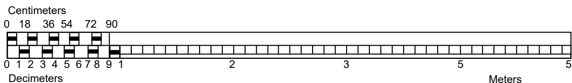
Figure 1.15: Vernier scale
