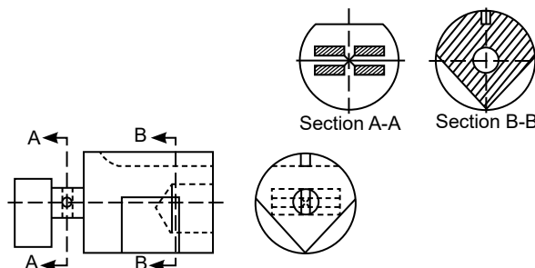
Figure 4.5: Removed Section
